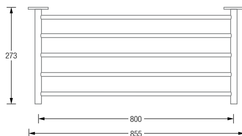
Product example SR800-1W-B Plan View:
