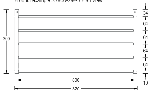
Product example SR800-2W-B Plan View:
