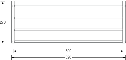
Product example G15-800-B Plan View:
