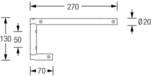
Product example G15-800-B Side View:
