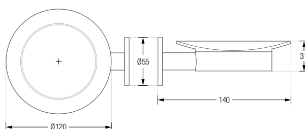
ATSOL-K55 Top / Side View:
