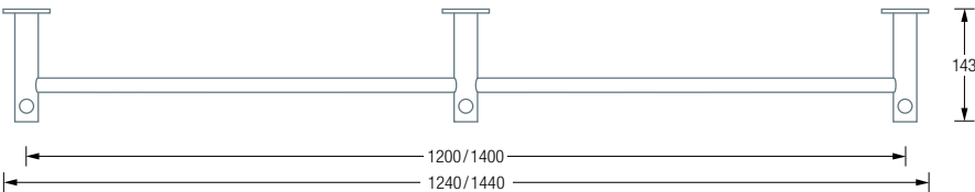
G4-1200 / 1400 Plan View:
