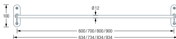
KLR600 / 700 / 800 / 900 Front View Folded:
