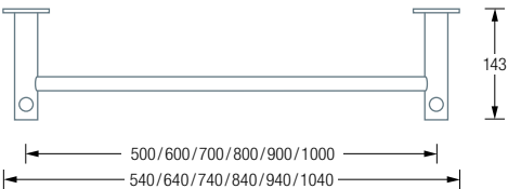
G4-500 / 600 / 700 / 800 / 900 / 1000 Plan View:
