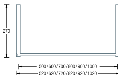
G13-500 / 600 / 700 / 800 / 900 / 1000 Plan View:
