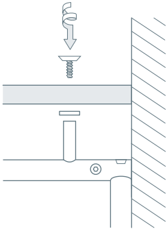
Assembly of wooden shelf:
