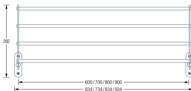
Installation with oval rosette:
