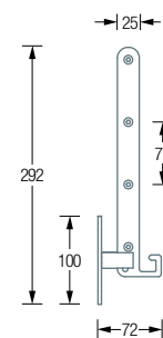
KLR600 / 700 / 800 / 900 Side View Folded:
