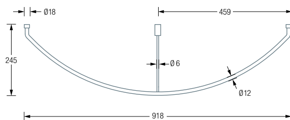
Mounting with mounting sleeve and wall bracket STF:
