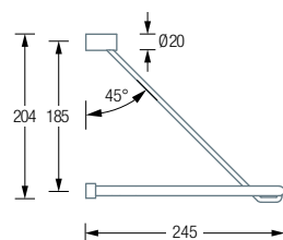
G45 Side View
