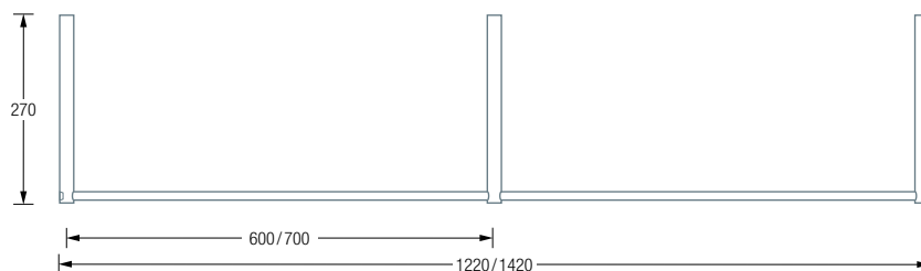
G13-1200 / 1400 Plan View:
