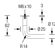
Product example HS12-800G Detail view:
