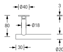
Product example HS18-800T Detail view:
