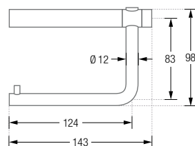
TPH4 Front View:
