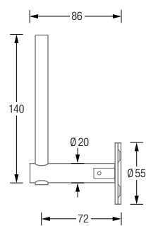
RTPH2-140 Side View:
