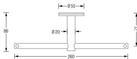
TPH3-260D Top View:
