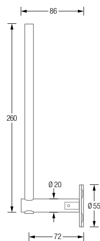
RTPH2-260D Side View:
