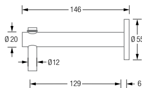
TPH1-K55 Side View:
