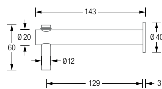
TPH1 Side View:
