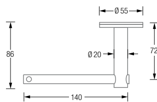
TPH3-140 Top View:
