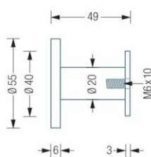
Wall mounting with rosette:
