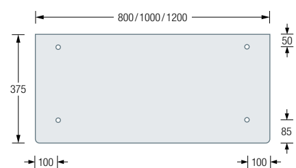
GL2G-SR600/SR800/ SR1000 Top View:
