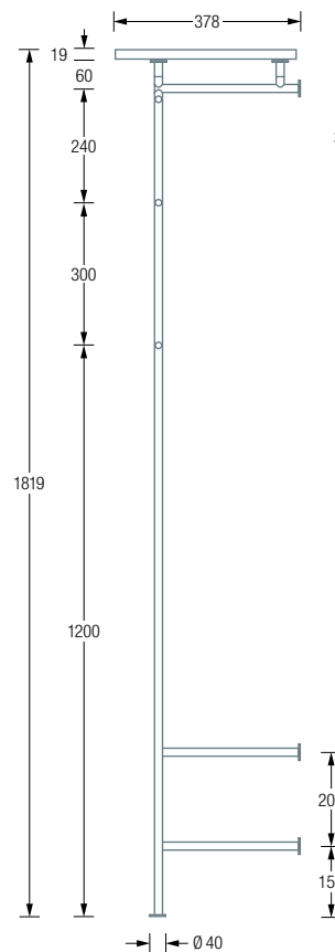
GL2-Oak-SR600/SR800/ SR1000 Side View:
