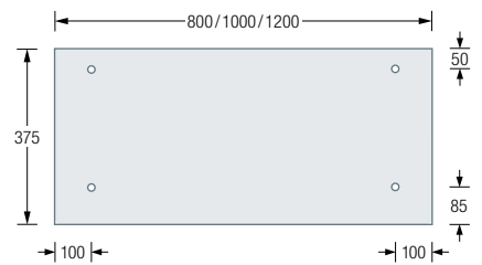
GL2-Oak-SR600/SR800/ SR1000 Top View:
