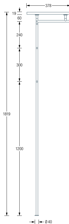
GL2-Oak-600/800/ 1000 Side View:
