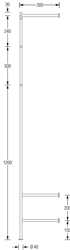
GL2-SR600/SR800/SR1000 Side View:
