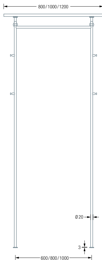
GL2-Oak-600/800/ 1000 Front View:
