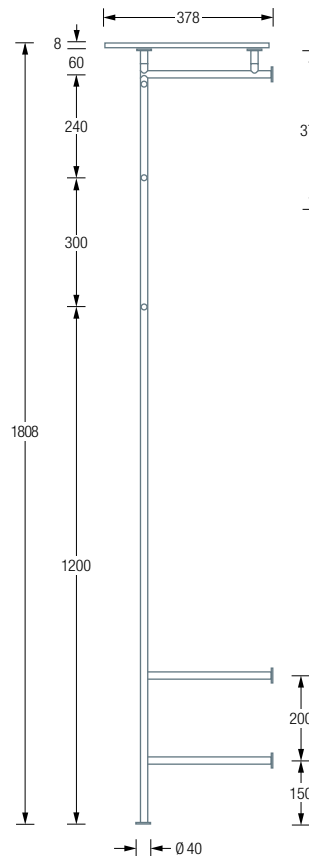
GL2G-SR600/SR800/ SR1000 Side View:
