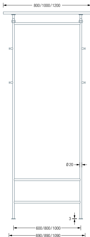
GL2-Oak-SR600/SR800/ SR1000 Front View:
