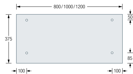
GL2-Oak-600/800/ 1000 Top View:
