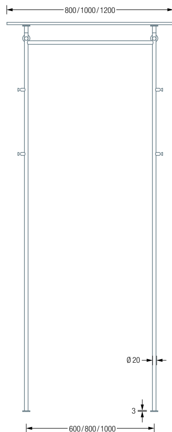
GL2G-600 / 800 / 1000 Front View:
