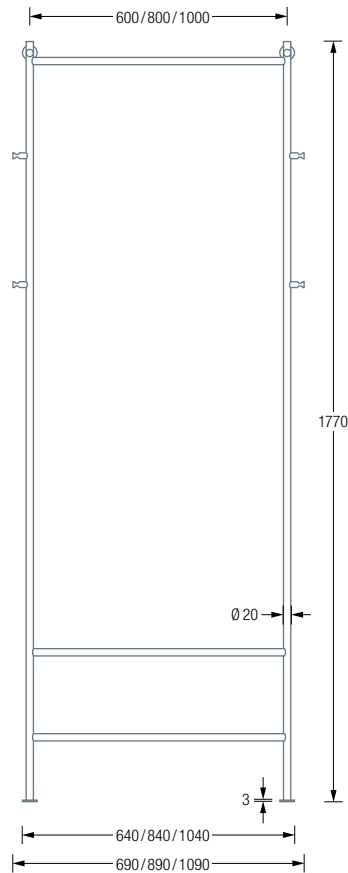
GL2-SR600/SR800/SR1000 Front View:
