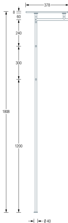
GL2G-600 / 800 / 1000 Side View:
