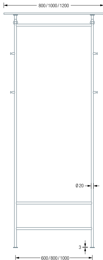
GL2G-SR600/SR800/ SR1000 Front View:
