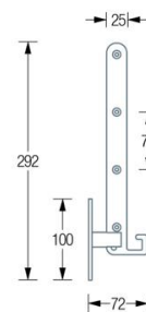
KLR600 / 700 / 800 / 900 Side View Folded:
