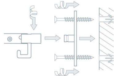
Installation with oval rosette:
