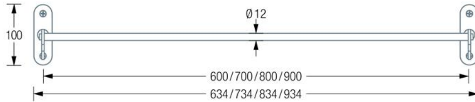
KLR600 / 700 / 800 / 900 Front View Folded:
